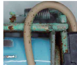
Yoke armature
