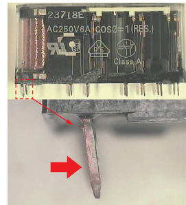
Deformation of the relay terminal
