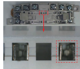
Deformation of the socket terminal
