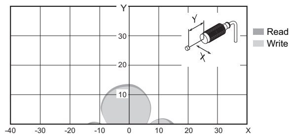
● V680-HS52 (Embedded in Metal) and V680-D1KP53M
