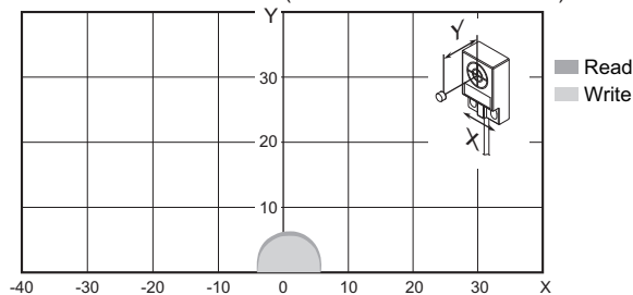
● V680-HS61 (with Non-Metal on Back Surface) and V680-D1KP52MT (Embedded in Metal: Steel)
