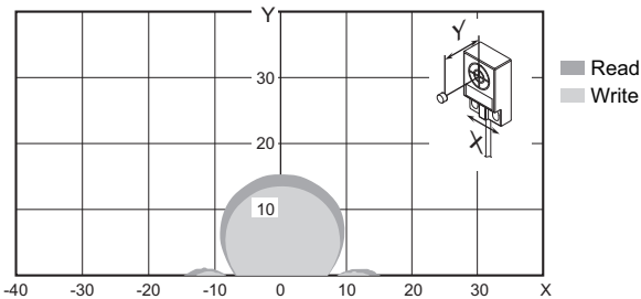
● V680-HS61 (with Non-Metal on Back Surface) and V680-D1KP52MT
