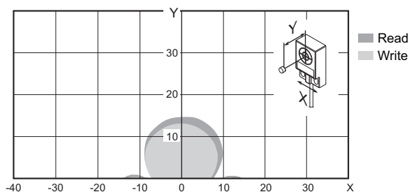
● V680-HS61 (with Non-Metal on Back Surface) and V680-D1KP53M
