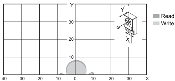
● V680-HS61 (with Non-Metal on Back Surface) and V680-D1KP53M (Embedded in Metal: Steel)
