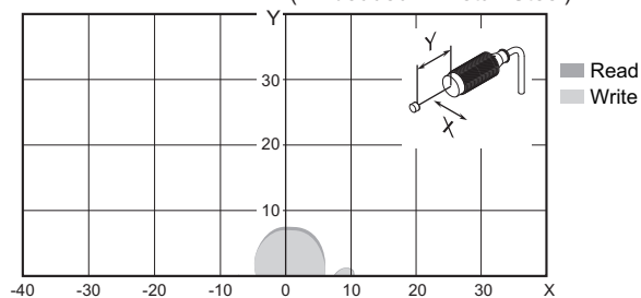
● V680-HS52 (Embedded in Metal) and V680-D1KP53M (Embedded in Metal: Steel)
