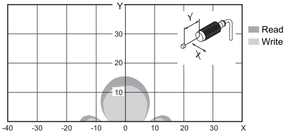
● V680-HS52 (Embedded in Metal) and V680-D1KP52MT
