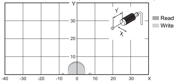
● V680-HS52 (Embedded in Metal) and V680-D1KP52MT (Embedded in Metal: Steel)
