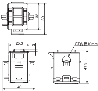
KM20-CTF-200A
