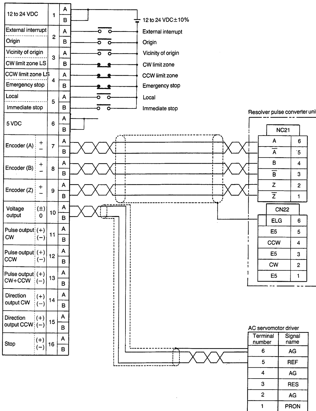
Position control unit:
