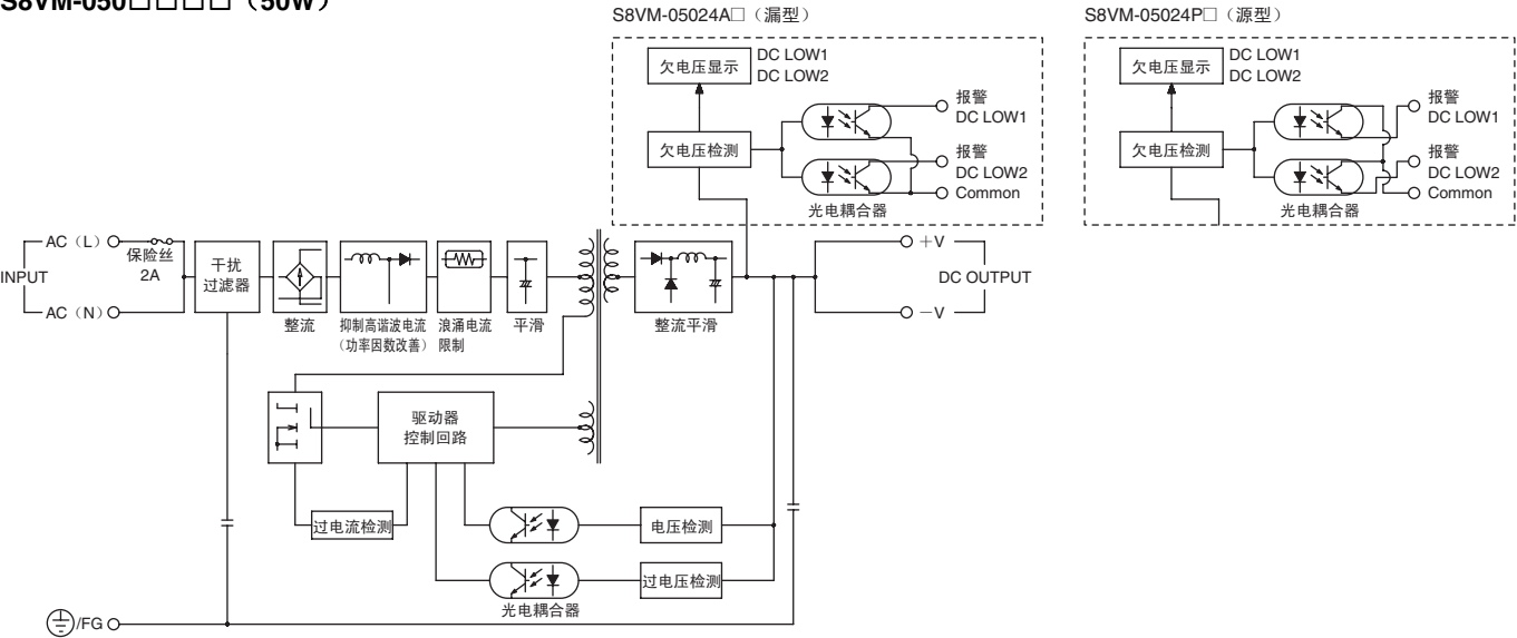
S8VM-050□□□□ (50W)
