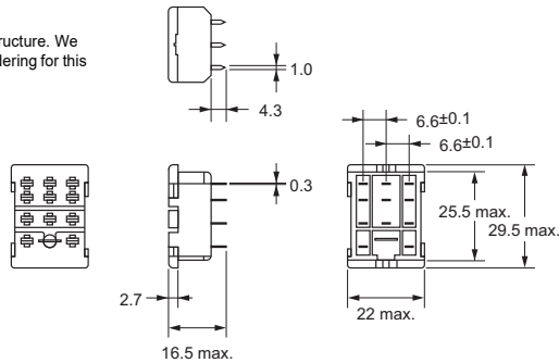
Terminal Arrangement/Internal Connection Diagram
