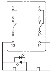
(Coil has no polarity)
