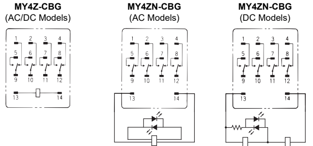
(The coil has no polarity.) (The coil has no polarity.) (The coil has no polarity.)
