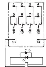
(Coil has no polarity)
