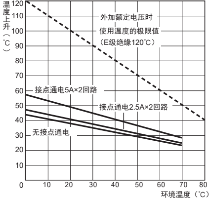
MY4□□-□□GS-R AC规格50Hz
