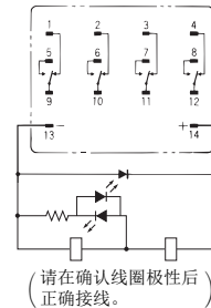
LY4N-D2
