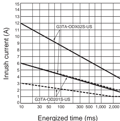
G3TA-ODX02S/OD201S-US
