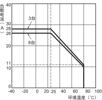
G3PE-235B (L)
