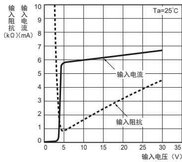
G3PE-2□□B
