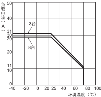
G3PE-545B (L)
