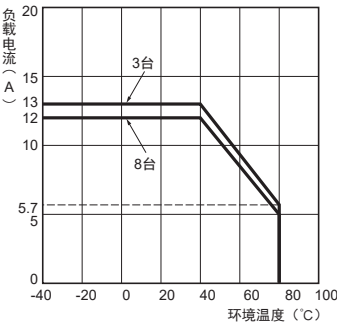
G3PE-515B (L)
