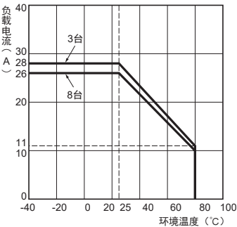
G3PE-535B (L)
