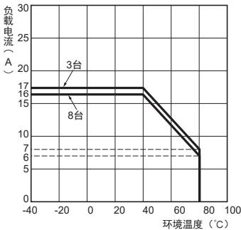
G3PE-525B (L)
