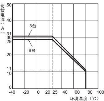
G3PE-245B (L)
