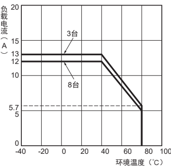
G3PE-215B (L)
