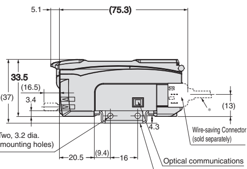
With Mounting Bracket Attached
