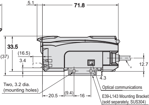
Mounting Holes
