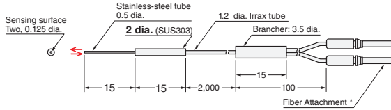
23-D E32-D331 2M (No Cutting)
