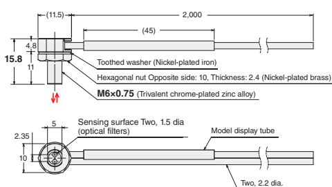
11-G E32-LR11NP 2M (Free Cutting)
