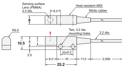
(29-D) E32-T14 2M (Free Cutting)
