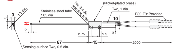
23-L E32-D25-S3 2M (Free Cutting)
