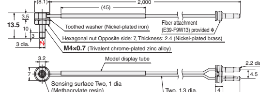
11-E E32-D21N 2M (Free Cutting)
