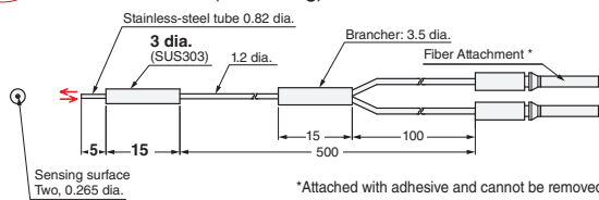
23-F E32-D32-S1 0.5M (No Cutting)
