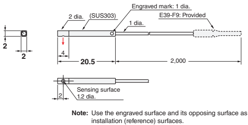
35-C E32-A04 2M (Free Cutting)
