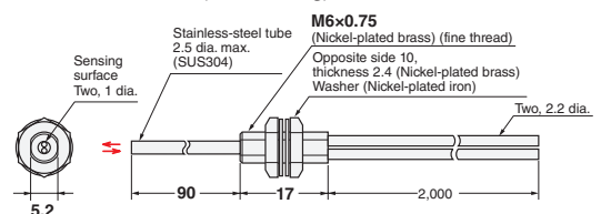
23-K E32-DC200BR 2M (Free Cutting)
