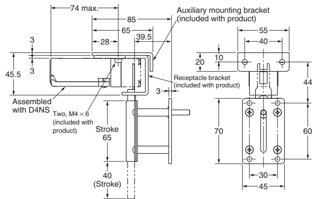
Switch Mounting Pattern 1
