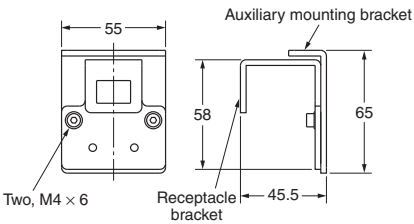
Auxiliary Mounting Bracket and Receptacle Bracket
