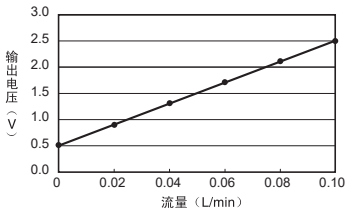
D6F-P0001A1
