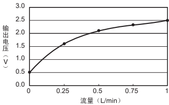
D6F-P0010A1/-P0010A2/-P0010AM2
