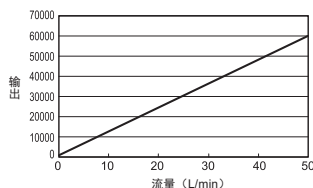
D6F-10A7D-000-0
