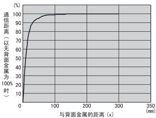
● V680S-HMD66-PNT & V680S-D8KF67
