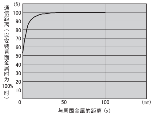
● V680S-HMD64-PNT & V680S-D8KF68M
