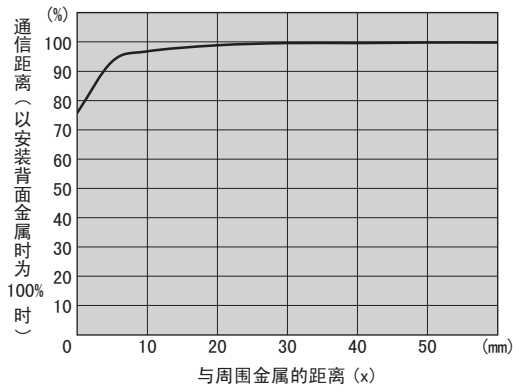
● V680S-HMD66-PNT & V680S-D2KF67M
