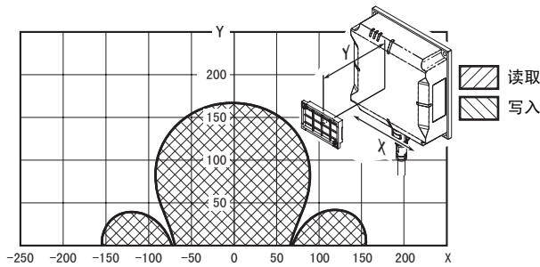
● V680S-HMD66-PNT & V680S-D8KF68 (背面: 金属) (RF 标签横向)
