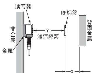
● V680S-HMD66-PNT & V680S-D8KF67
