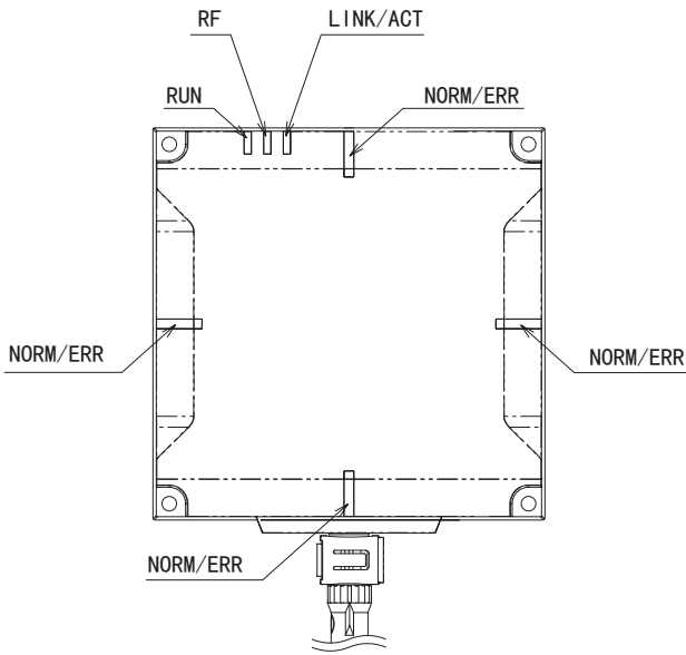
V680S-HMD66-PNT
