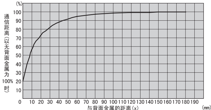
● V680S-HMD66-PNT & V680-D1KP58HTN
