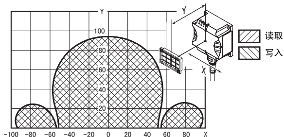
● V680S-HMD64-PNT & V680S-D2KF68M (背面: 金属) (RF 标签横向)
