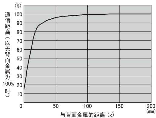
● V680S-HMD64-PNT & V680S-D2KF67
