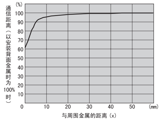
● V680S-HMD64-PNT & V680S-D8KF67M
