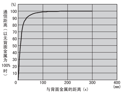
● V680S-HMD66-PNT & V680S-D2KF67
