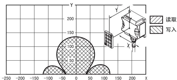
● V680S-HMD64-PNT & V680S-D8KF68M (背面: 金属) (RF 标签纵向)
