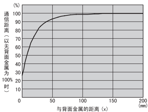
● V680S-HMD64-PNT & V680S-D2KF68
