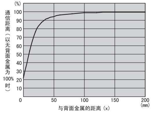
● V680S-HMD66-PNT & V680-D8KF68A
