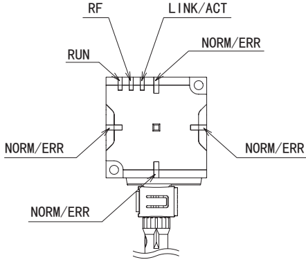
V680S-HMD63-PNT
