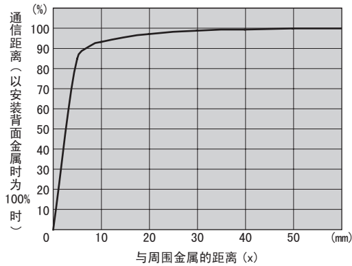
● V680S-HMD66-PNT & V680S-D2KF67M
