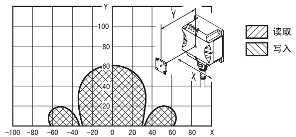
● V680S-HMD64-PNT & V680S-D8KF67M (背面: 金属) (背面: 金属)
