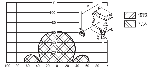
● V680S-HMD64-PNT & V680-D8KF68A (背面: 金属) (RF 标签纵向)
