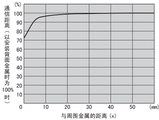
● V680S-HMD66-PNT & V680S-D8KF67M
