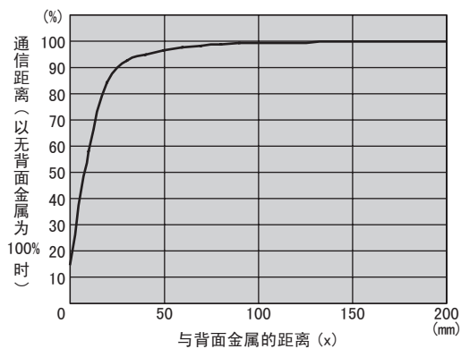
● V680S-HMD64-PNT & V680S-D8KF67
