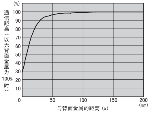
● V680S-HMD64-PNT & V680-D8KF68A
