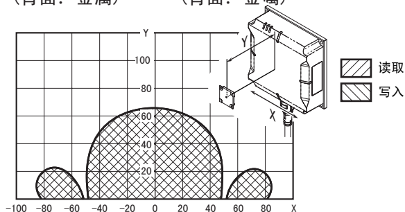
● V680S-HMD66-PNT & V680S-D8KF67M (背面: 金属) (背面: 金属)
