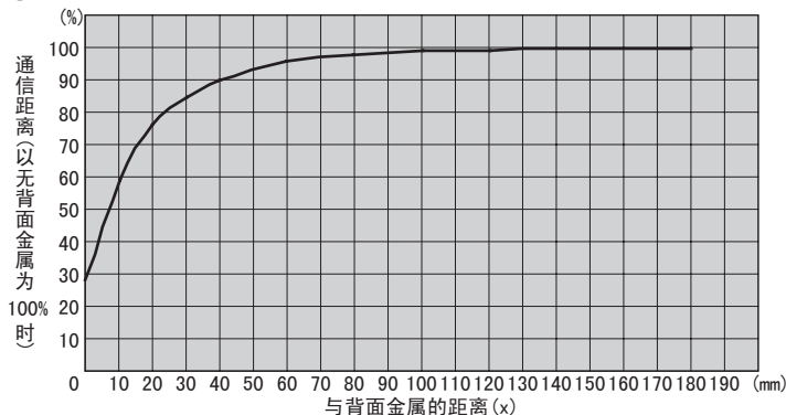
● V680S-HMD64-PNT & V680-D1KP58HTN
