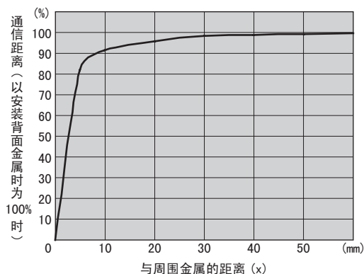
● V680S-HMD66-PNT & V680-D8KF67M
