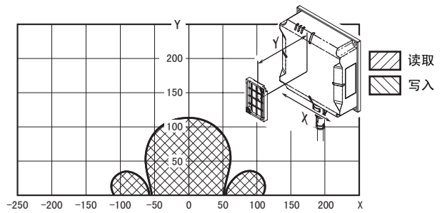
● V680S-HMD66-PNT & V680S-D2KF68M (背面: 金属) (RF 标签纵向)
