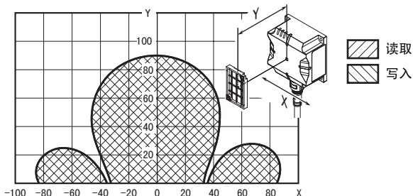
● V680S-HMD64-PNT & V680S-D8KF68M (背面: 金属) (RF 标签纵向)
