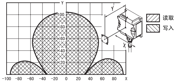
● V680S-HMD64-PNT & V680S-D8KF67 (背面: 金属)
