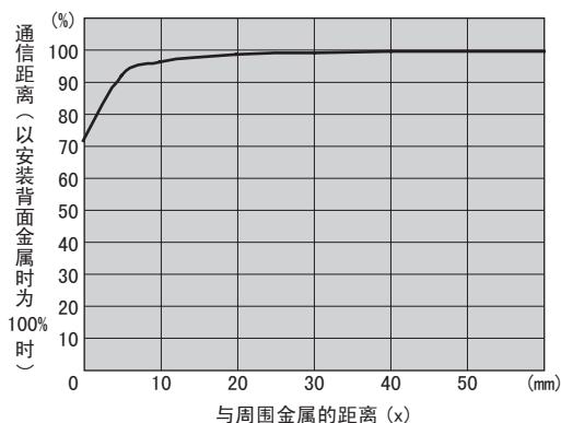
● V680S-HMD64-PNT & V680-D8KF67M
