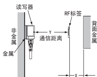
● V680S-HMD66-PNT & V680S-D2KF67
