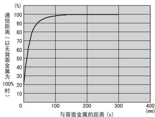
● V680S-HMD66-PNT & V680S-D2KF68
