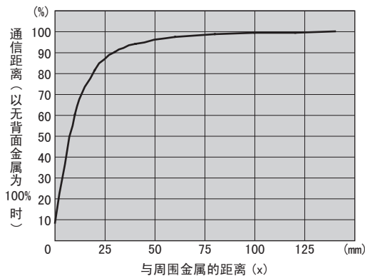
● V680S-HMD64-PNT & V680-D8KF67
