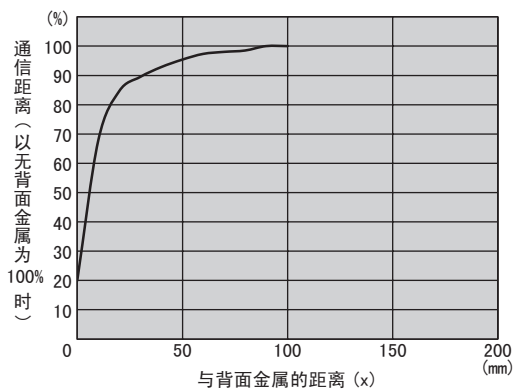
● V680S-HMD63-PNT & V680S-D2KF67
