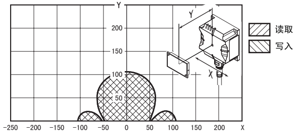
● V680S-HMD64-PNT & V680S-D2KF67 (背面: 金属)
