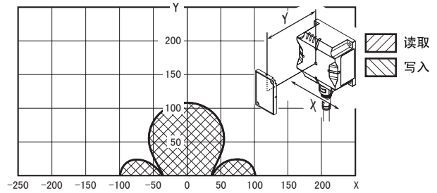
● V680S-HMD64-PNT & V680S-D2KF67M (背面: 金属) (背面: 金属)
