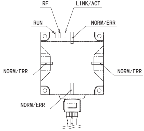
V680S-HMD64-PNT
