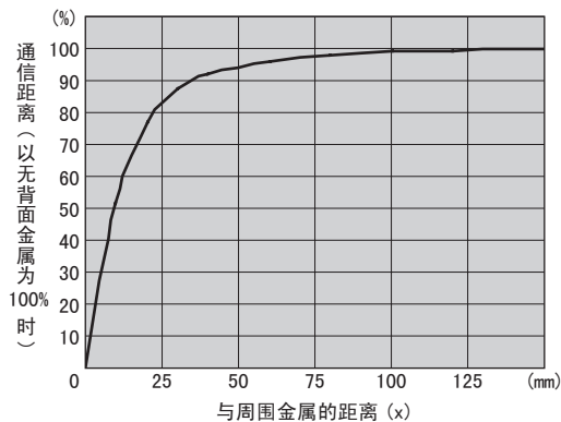
● V680S-HMD66-PNT & V680-D8KF67
