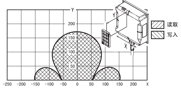
● V680S-HMD66-PNT & V680S-D2KF68 (背面: 金属) (RF 标签纵向)
