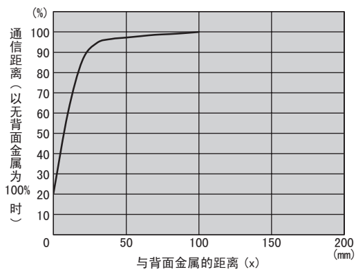
● V680S-HMD63-PNT & V680S-D8KF67
