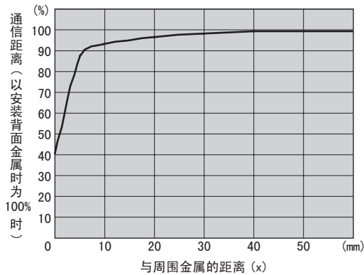
● V680S-HMD66-PNT & V680S-D8KF67M
