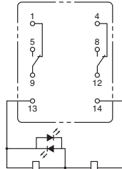
MY2IN(S) (DC规格)
